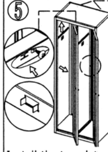
5 Install the top plate and fix it with screws(5x12)
