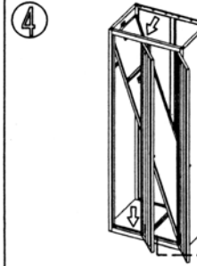
4 Install the bottom plate ,then fix the division plate as the sign
